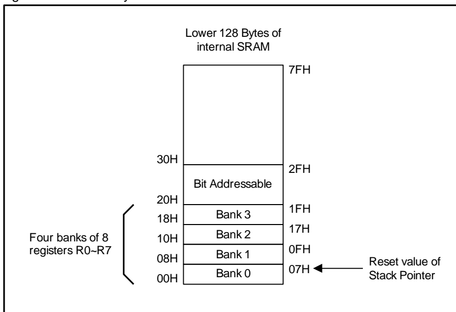
Fig 8-2 Lower 128 Bytes of Internal RAM
