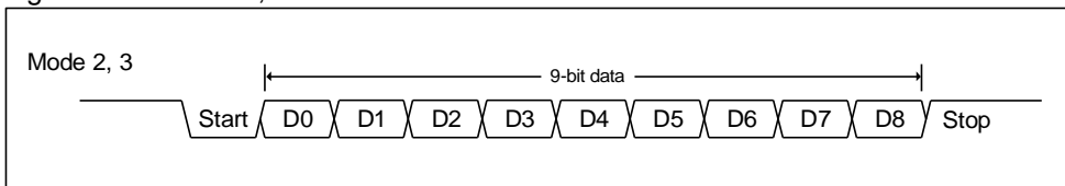
Figure 12-2 Mode 2, 3 Data Frame
