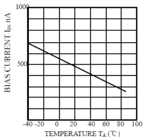
BIAS CURRENT-TEMPERATURE
