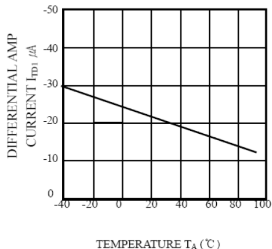
DIFFERENTIAL AMPLIFIER OUTPUT CURRENT-TEMP
