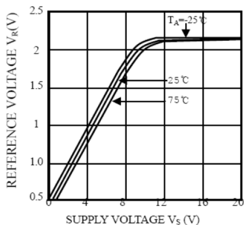
REFERENCE VOLTAGE-SUPPLY VOLTAGE
