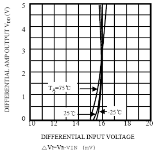
DIFFERENTIAL AMPLIFIER OUTPUT VOLTAGE - DIFFERENTIAL INPUT VOLTAGE
