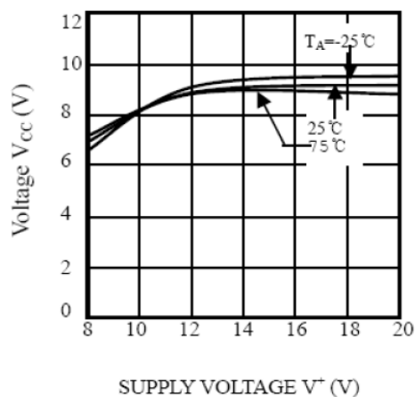
VOLTAGE-SUPPLY VOLTAGE
