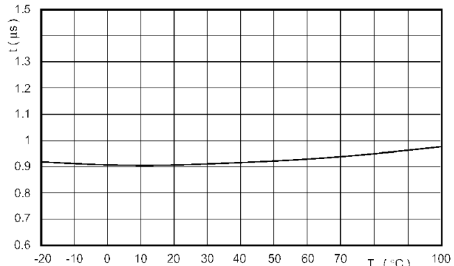
Trigger pulse width (90% amplitude) vs. temperature, V CC = 10 V
