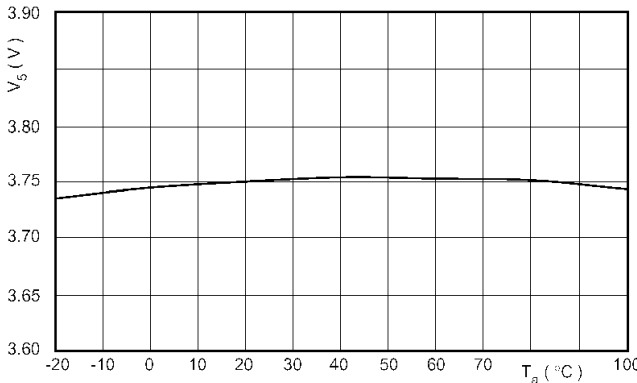
Static overload threshold V CC = 10 V
