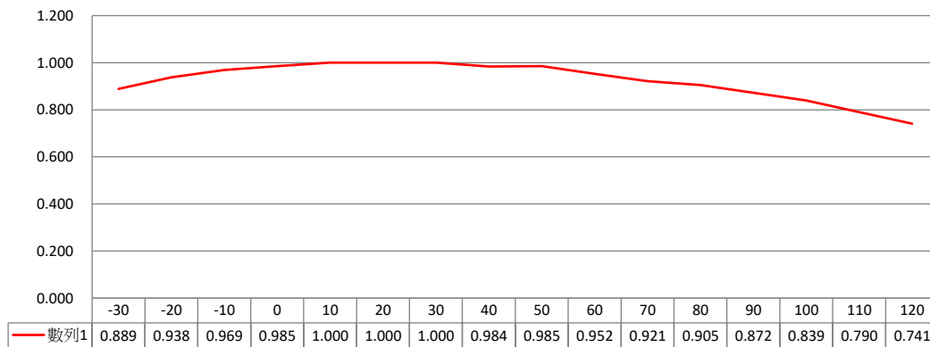
WCS2750 Sensitivity standardization of 30°C (5V) V.S Temperature
