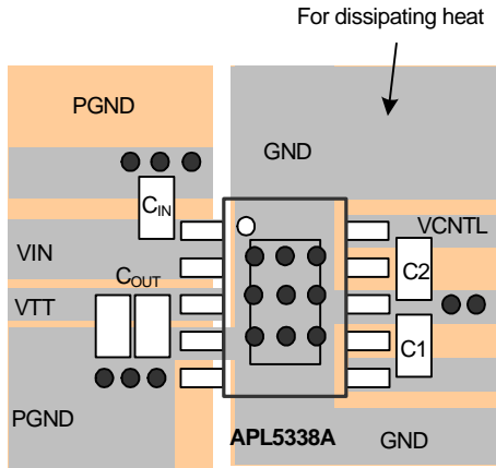
Figure 2. Recommended Layout
