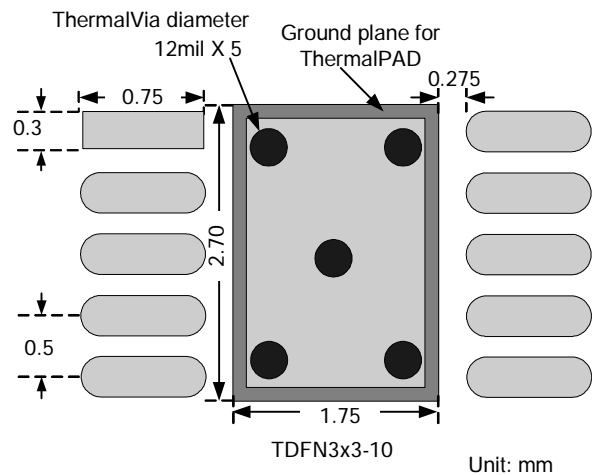
APW8805A Recommended Footprint
