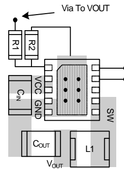
APW8805A Layout Consideration
