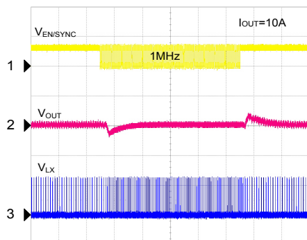
SYNC Transient
