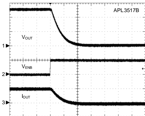
Shutdown Response
