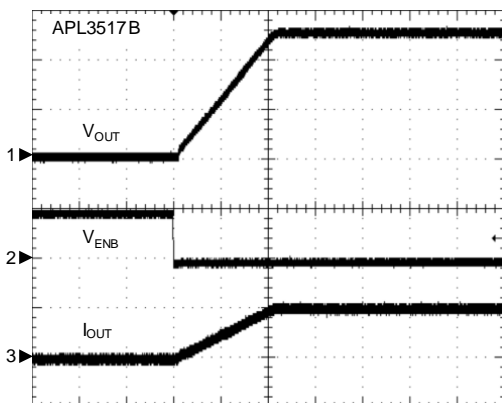
Enable Response
