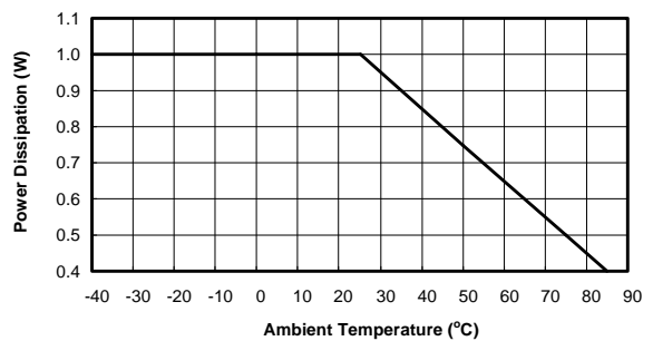
Figure 2. Derating Curves for APL3527S Package
