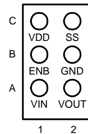
WLCSP1.16x0.76-6 (Top View)
