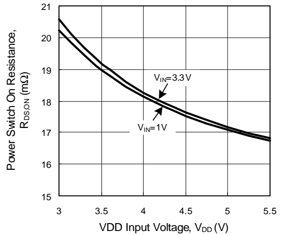
Power Switch On Resistance vs. VDD Input Voltage
