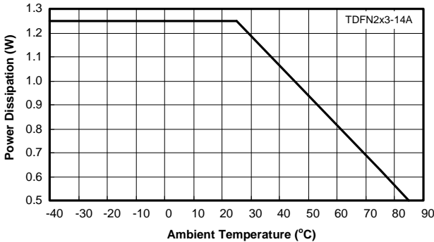
Figure 3. Derating Curves for APL3528 Package
