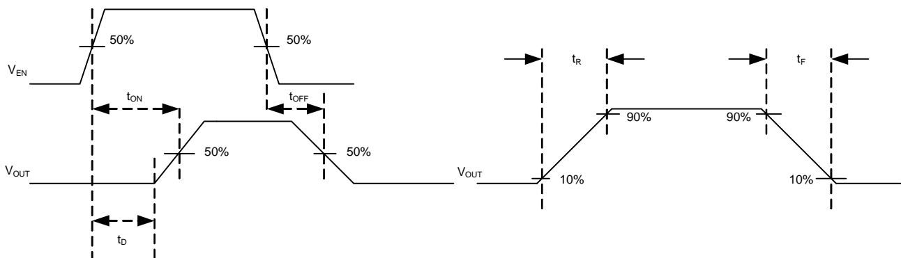
Figure 1. t_{ON}/t_{OFF}, t_d/t_R/t_F Waveforms
