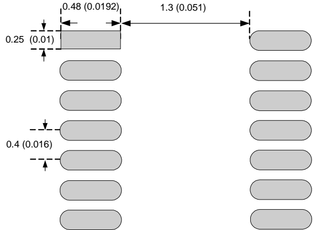
TDFN2x3-14A
