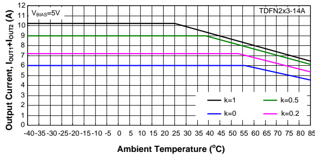
Figure 3. Derating Curves for APL3533 Package
