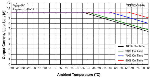
Figure 4. Safe Operating Area for APL3533 Package
