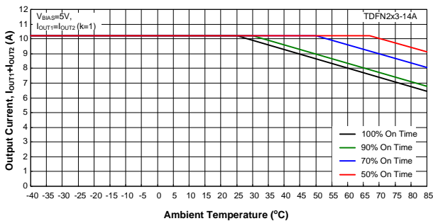
Figure 4. Safe Operating Area for APL3533A Package
