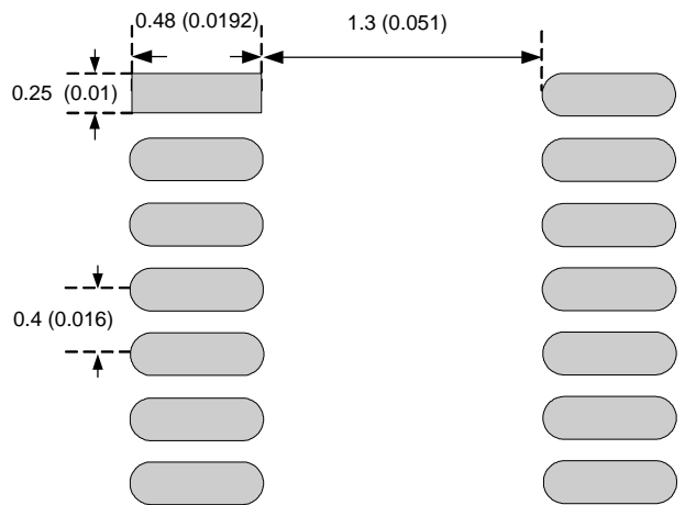
TDFN2x3-14A
