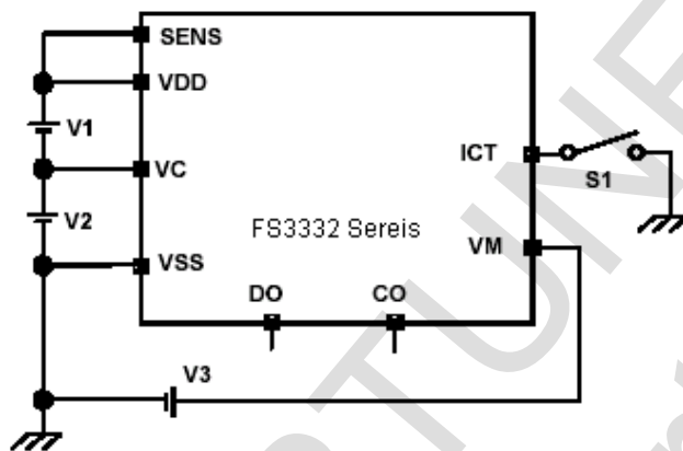
Measurement circuit 1
