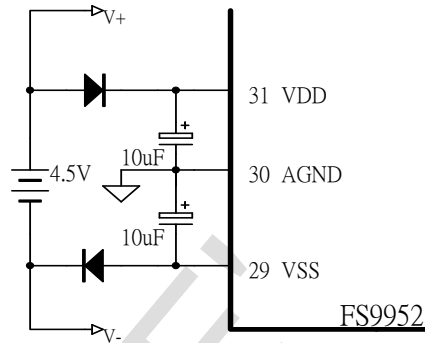
Diagram 17 4.5V Power Supply
