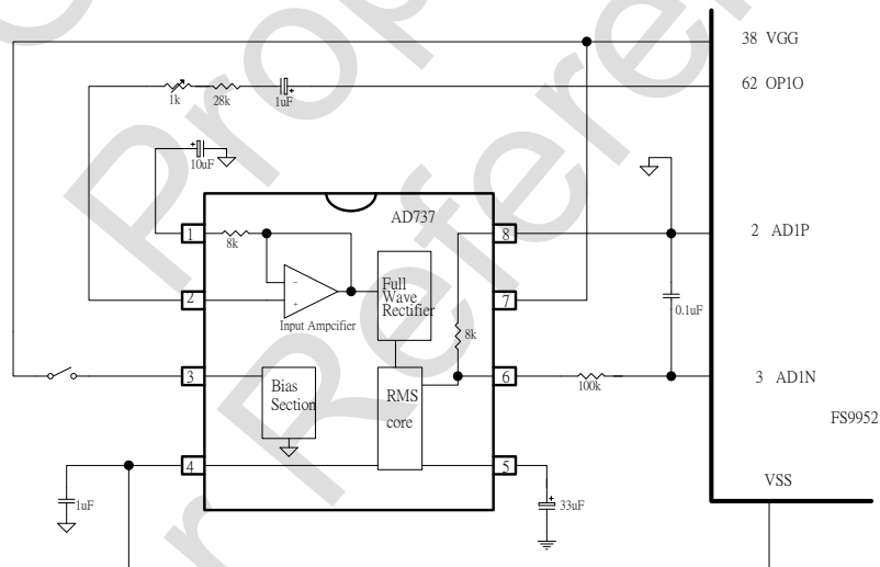
Diagram 24 True Valid Value Rectification Circuit
