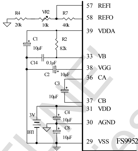
Diagram 7 Power System
