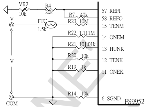
Diagram 25 Voltage Measurement
