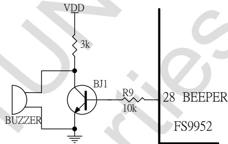
Diagram 15 High Resistance Buzzer Connection
