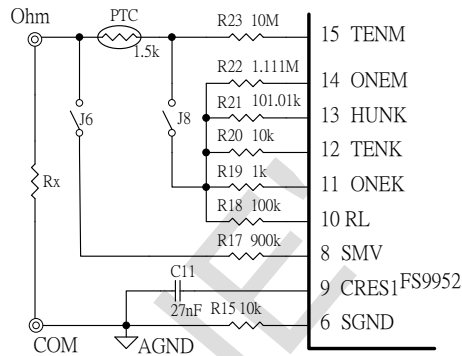
Diagram 28 Resistance Measurement
