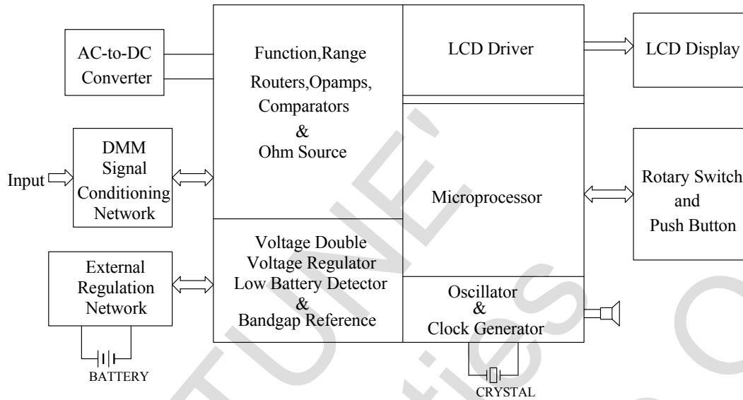
Diagram 1 Block Diagram
