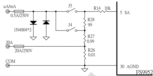
Diagram 27 Current Measurement
