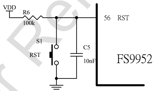
Diagram 13 Reset Keys
