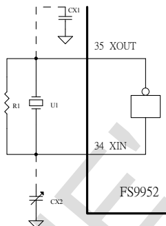
Diagram 9 Oscillation Circuit
