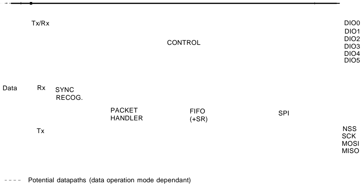
Figure 25. RFM95T/96T(W) Data Processing Conceptual View
