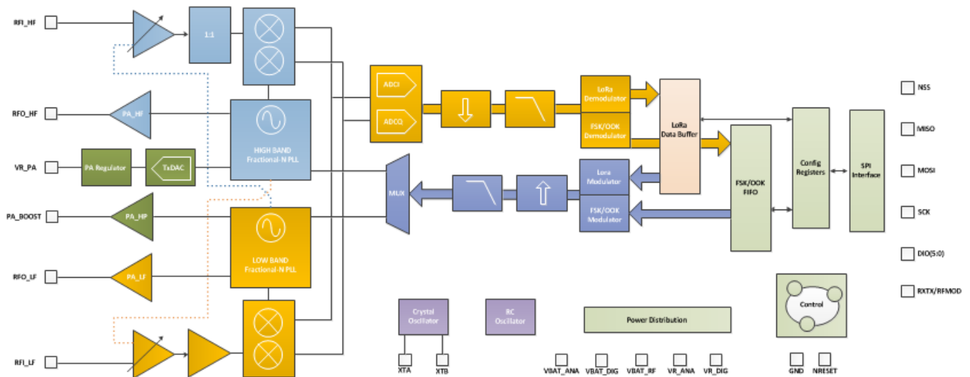
Figure 3. RFM95T/96T(W) Block Schematic Diagram
