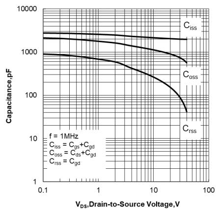
Figure 5. Capacitance Characteristics
