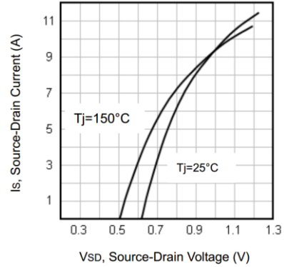
Figure 2. Forward Characteristic of Reverse Diode
