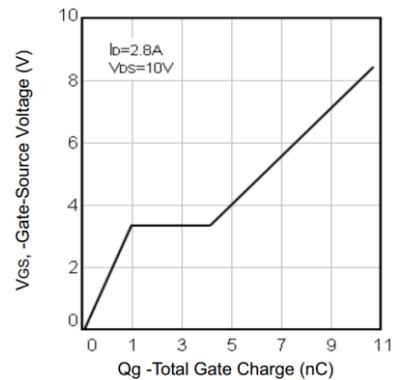
Figure 6. Gate Charge Characteristics
