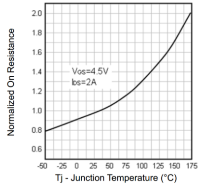
Figure 4. Normalized On-Resistance Vs Junction Temperature
