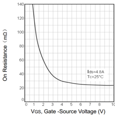
Figure 3. On-Resistance vs Gate Voltage
