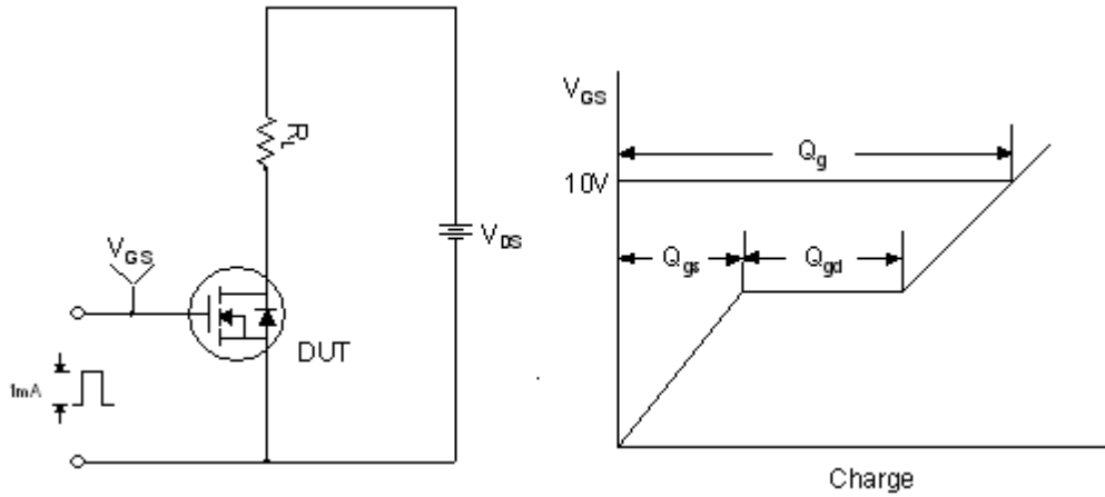
Figure 7. Gate Charge Test Circuit & Waveform
