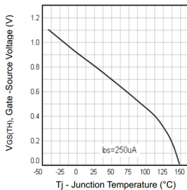
Figure 5. Gate Threshold Voltage vs Junction Temperature
