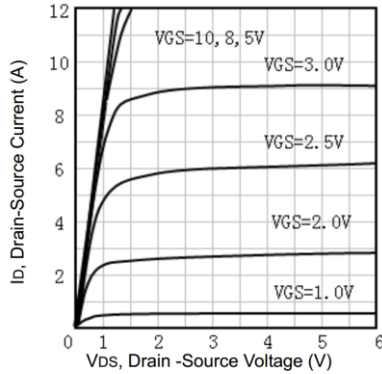
Figure 1. Output Characteristics
