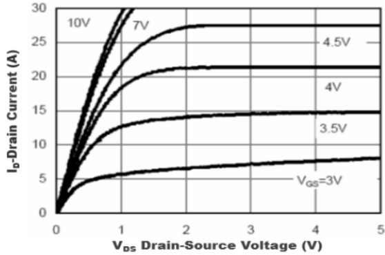
Figure 1. Output Characteristics
