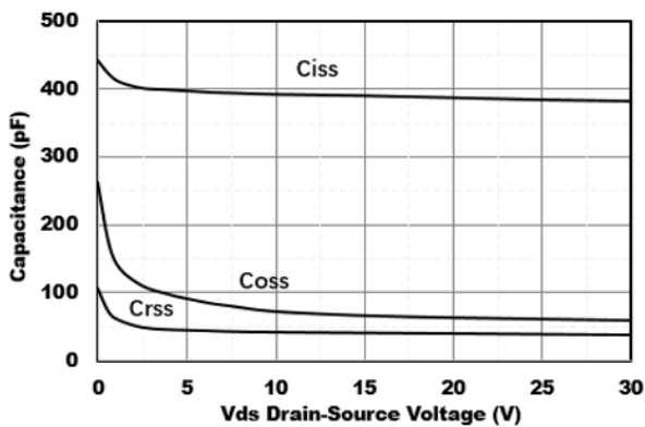
Figure 5. Capacitance Characteristics
