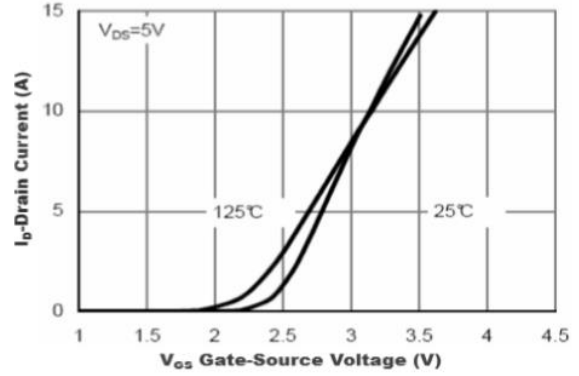
Figure 2. Transfer Characteristics
