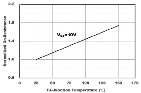
Figure 4. Drain-to-Source On Resistance
