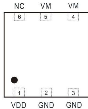
DFN2x2-6L
