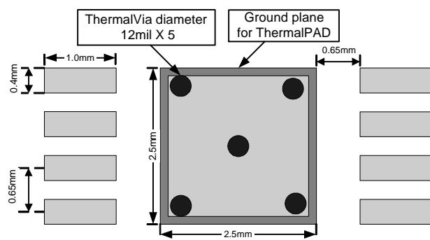
MSOP-8P Land Pattern Recommendation
