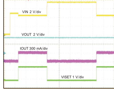
V_{IN} 0\text{V}-5\text{V}-7\text{V}-5\text{V} OVP from Normal Power-Up Operation
