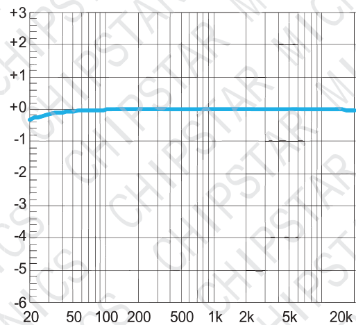
Figure 24. Frequency Response BTL mode, 3V, 80ohm
