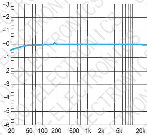
Figure 23. Frequency Response BTL mode, 5V, 80ohm
