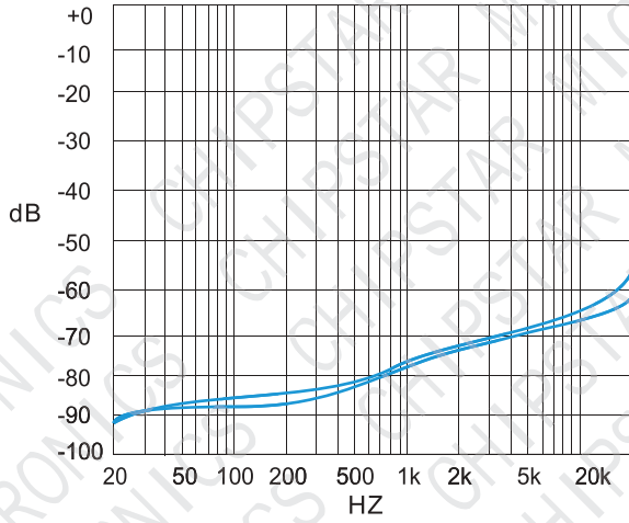
Figure 21. PSRR vs. Freq SE mode, 5V, 320ohm, 200mVpp Input unterminated
