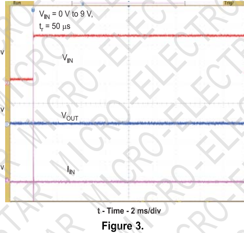
OVP RESPONSE FOR INPUT STEP
