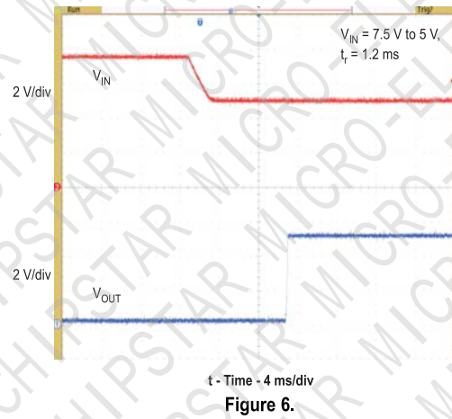
RECOVERY FROM OVP
