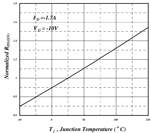
Fig 4. Normalized On-Resistance
