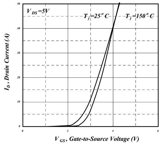
Fig 12. Transfer Characteristics
