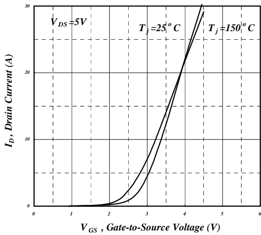
Fig 15. Transfer Characteristics
