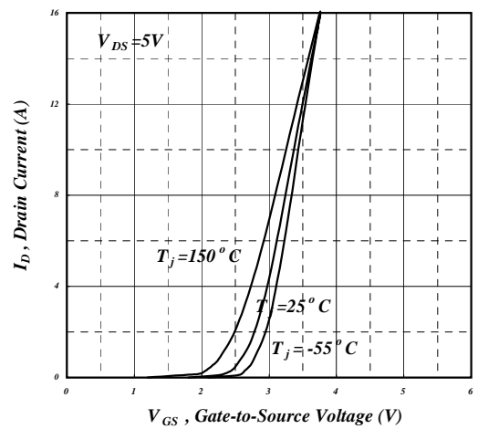
Fig 16. Transfer Characteristics
