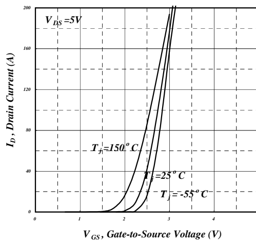
Fig 12. Transfer Characteristics
