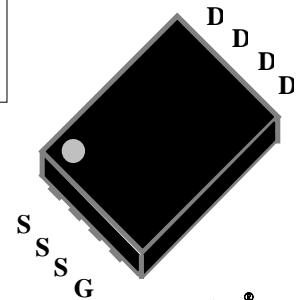
PMPAK ® 5x6
