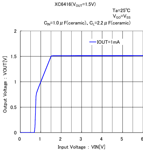
(2) Output Voltage vs. Input Voltage (Continued)
