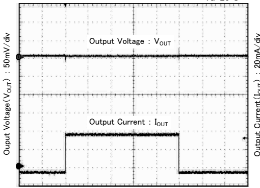
Time : 1ms/div
