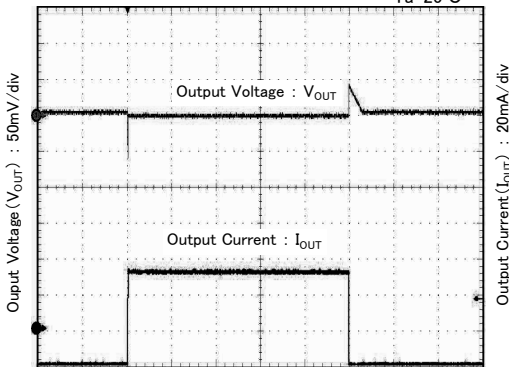
Time : 1ms/div
