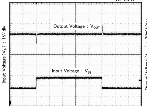
Time : 200 \mu s/div
