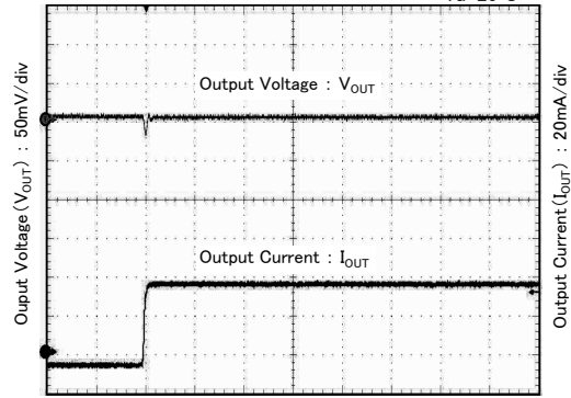
Time : 50 μs/div
