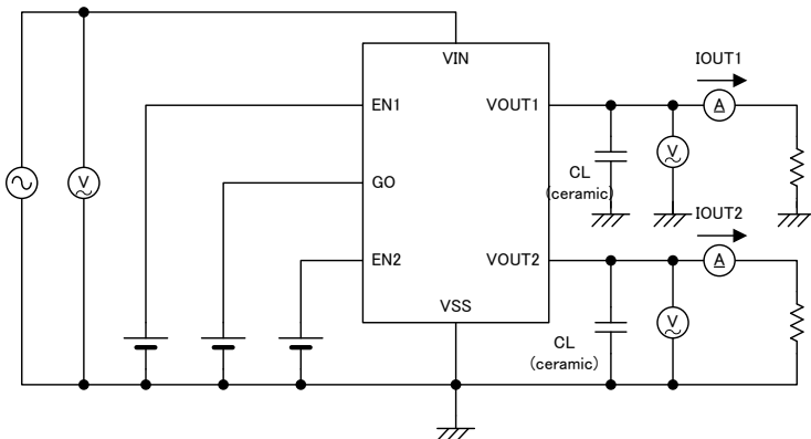
● Circuit ③
