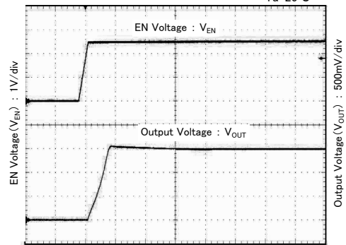
Time : 20 \mu s/div
