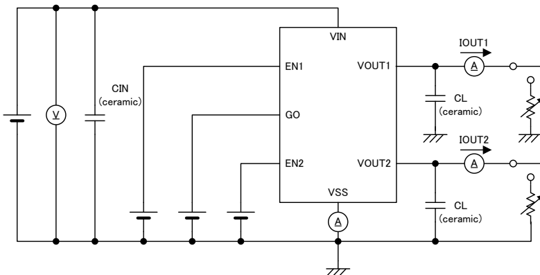
● Circuit ③
