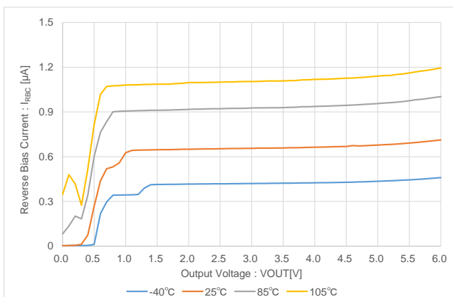
(4-1) Reverse Bias Current vs Output Voltage
