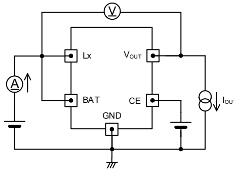
< Circuit No.④ >
