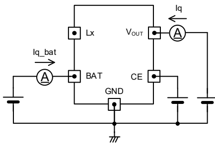
< Circuit No.③ >
