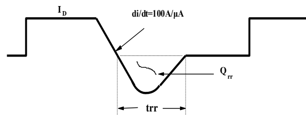
3) Diode Reverse Recovery Test Circuit & Waveform
