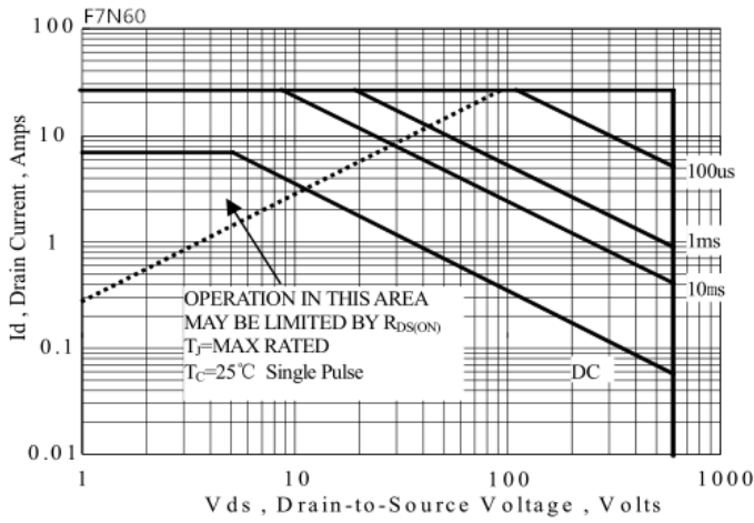
Figure 14 Maximum Forward Bias Safe Operating Area
