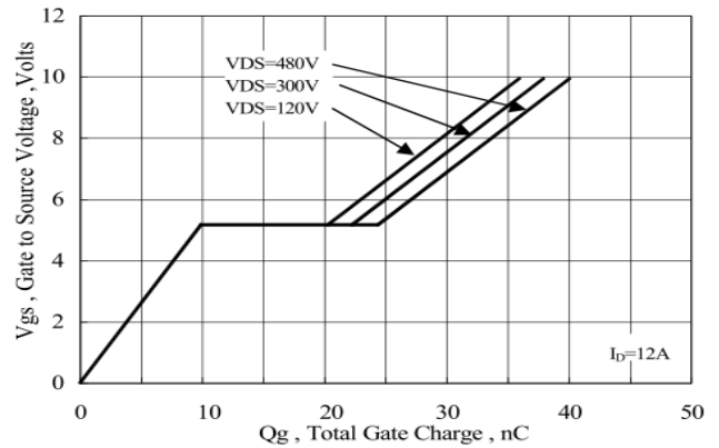
Figure 13 Typical Gate Charge vs Gate to Source Voltage
