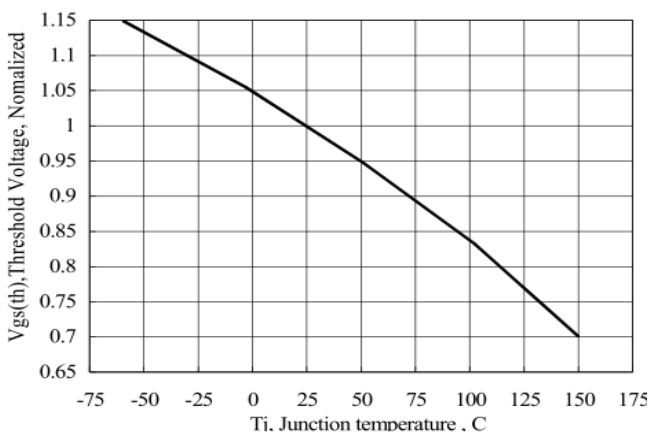
Figure 10 Typical Threshold Voltage vs Junction Temperature
