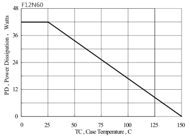
Figure 15 Maximum Power Dissipation vs Case Temperature
