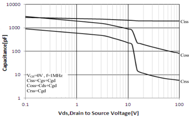
Figure 12 Typical Capacitance vs Drain to Source Voltage
