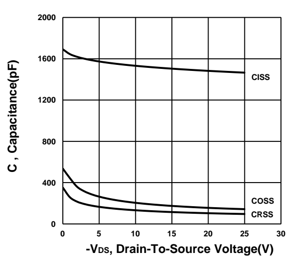
Capacitance Characteristic
