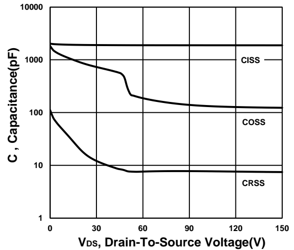
Capacitance Characteristic
