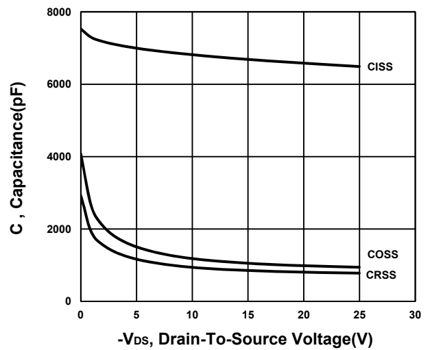
Capacitance Characteristic
