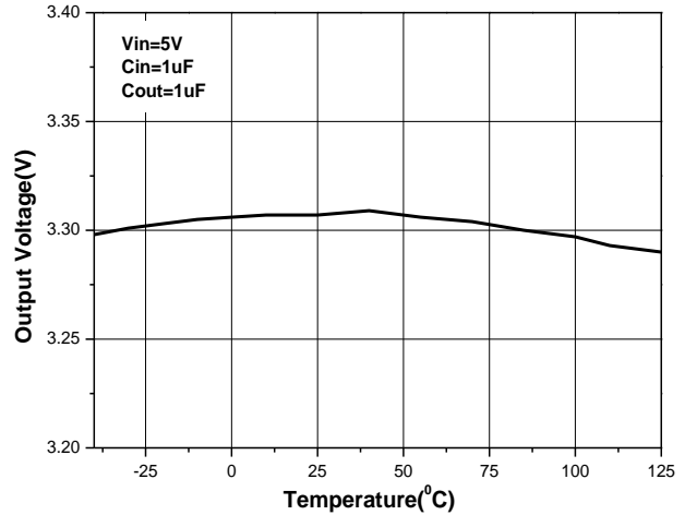
Figure 13. Temperature Stability
