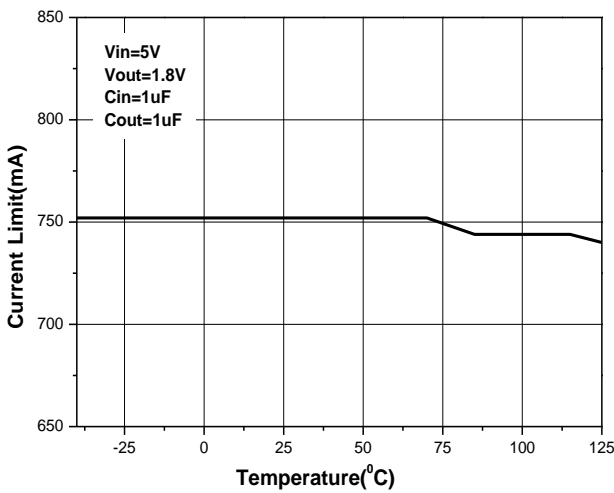
Figure 8. Current limit vs. Temperature
