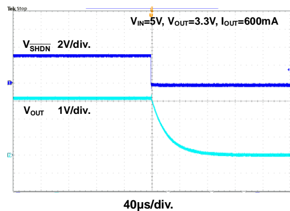
Figure 19. Shutdown Test
