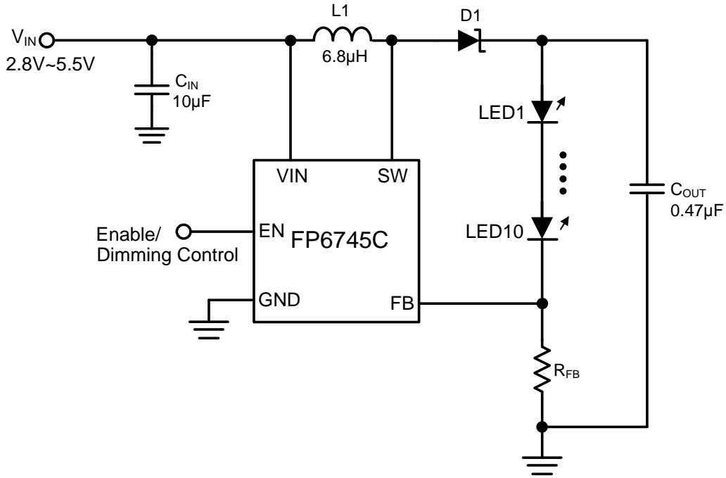
Figure 2. Typical Application Circuit of FP6745C
