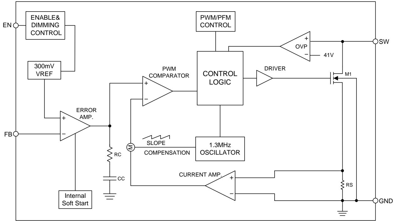
Figure 3. Block Diagram of FP6745C
