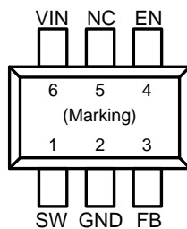
Figure 1. Pin Assignment of FP6745C
