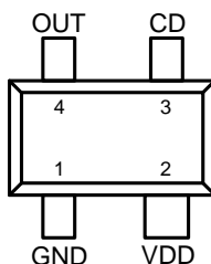
Figure 1. Pin Assignment of FP6801
