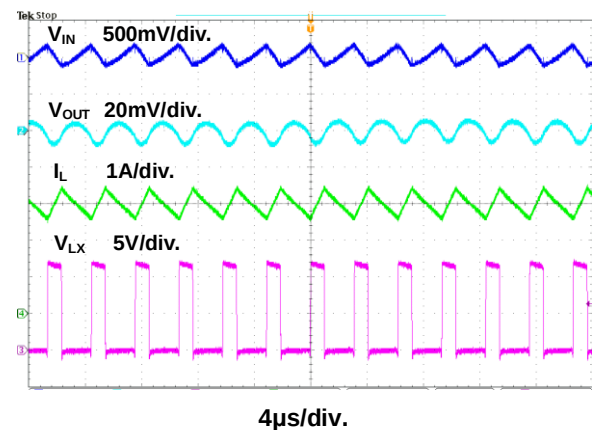
Figure 12. Steady State Waveform
