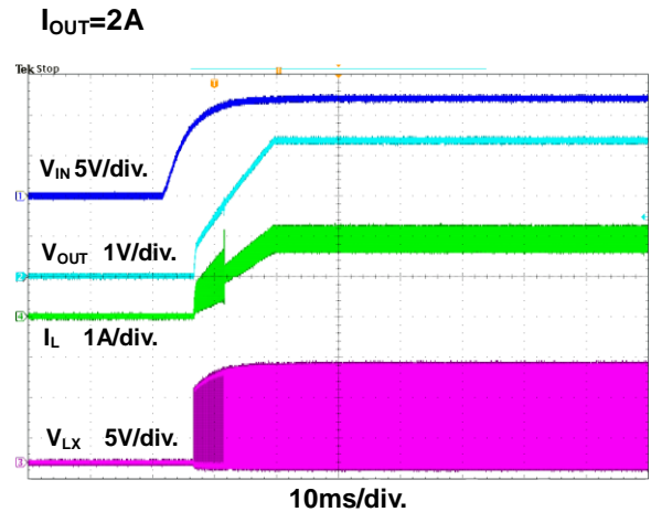
Figure 12. Power On through VIN Waveform
