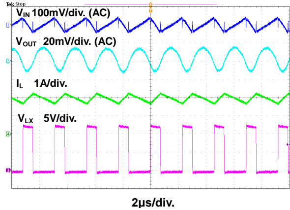
Figure 10. 2.5A Steady State Waveform
