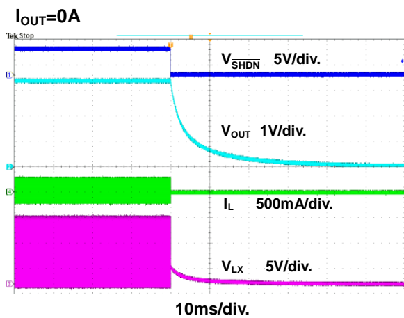
Figure 17. Power Off through \overline{SHDN} Waveform
