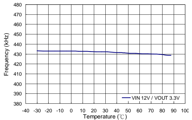
Figure 8. Frequency vs. Temperature
