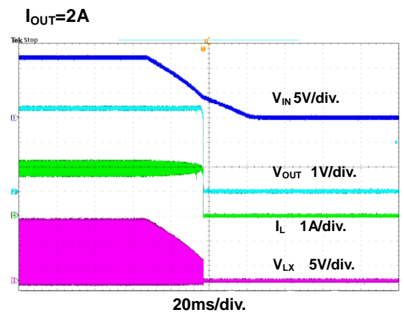
Figure 14. Power Off through VIN Waveform
