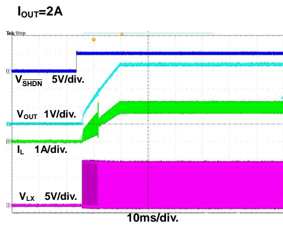
Figure 16. Power On through \overline{SHDN} Waveform
