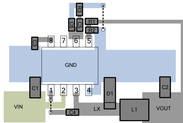
Figure 16. Recommended Layout Diagram
