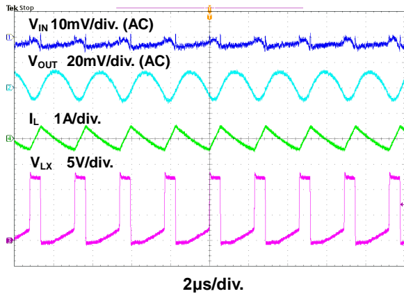
Figure 9. 0A Steady State Waveform
