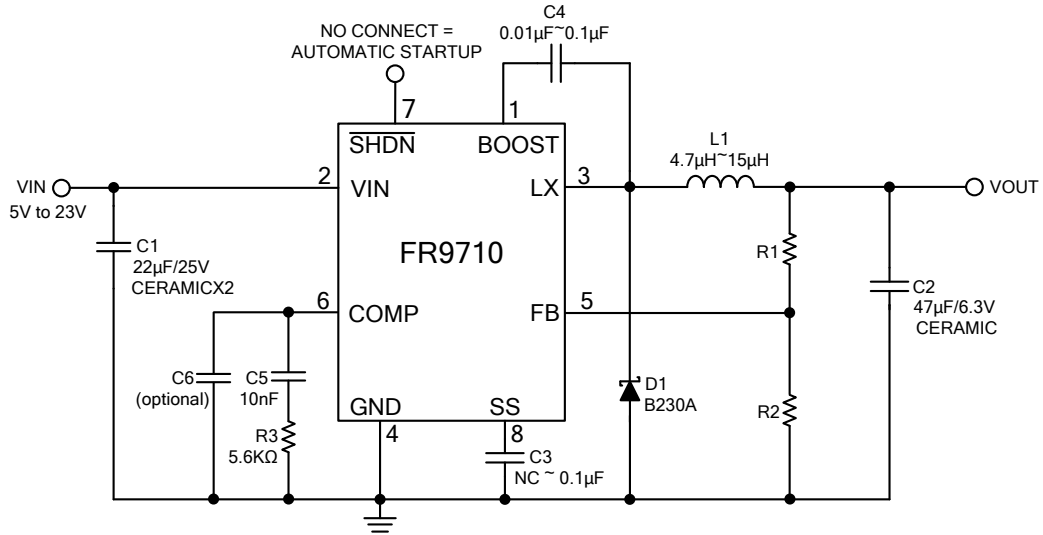
Figure 2. Output 3.3V Application Circuit
