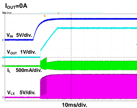
Figure 11. Power On through VIN Waveform
