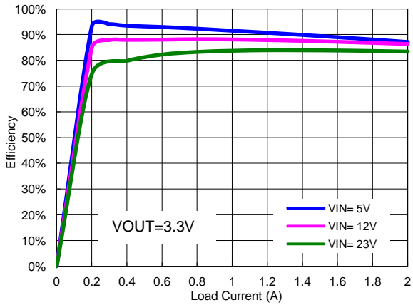
Figure 5. Efficiency vs. Loading
