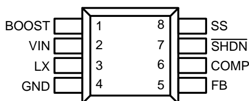
Figure 1. Pin Assignment of FR9710
