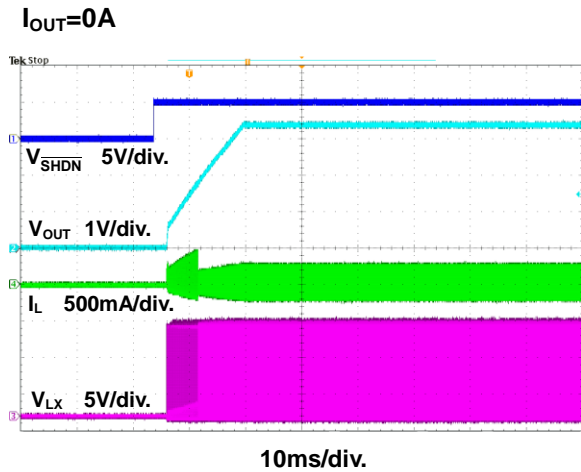
Figure 15. Power On through \overline{SHDN} Waveform
