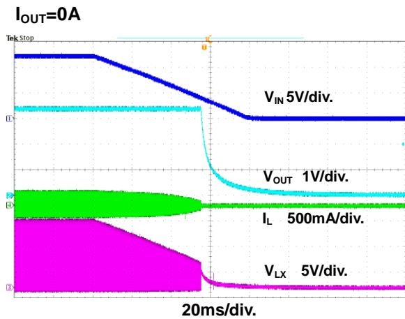
Figure 13. Power Off through VIN Waveform
