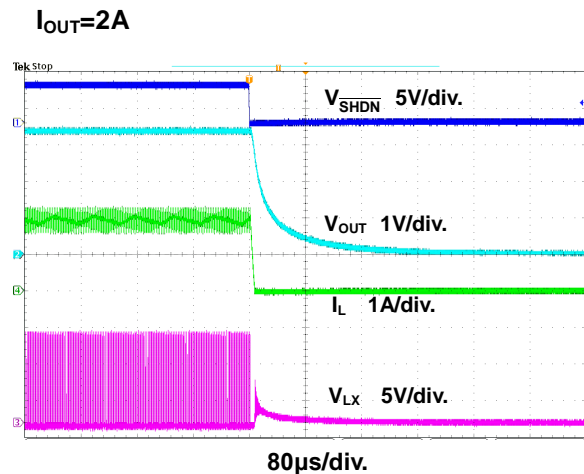
Figure 18. Power Off through \overline{SHDN} Waveform
