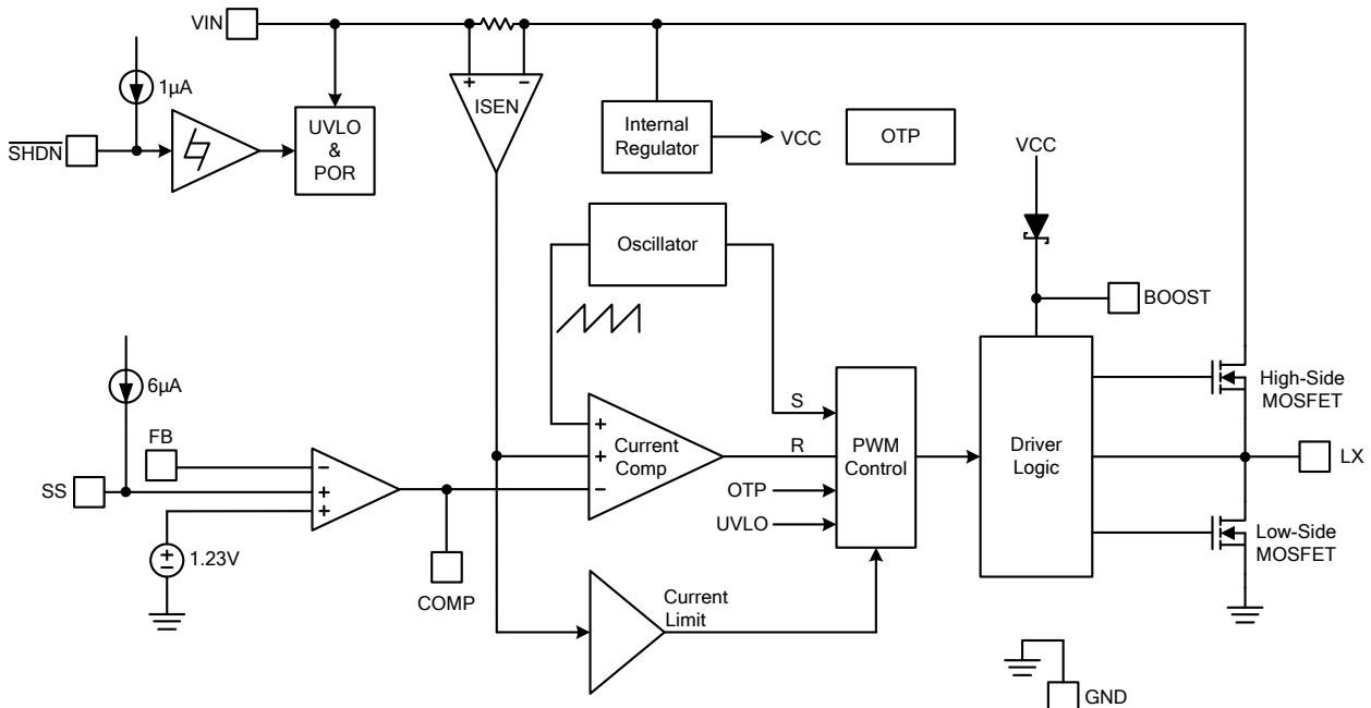
Figure 4. Block Diagram of FR9710
