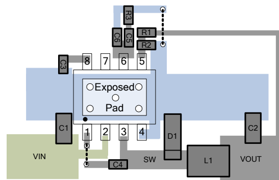
Figure 5. Recommended Layout Diagram
