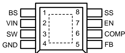
Figure 1. Pin Assignment of FR9723
