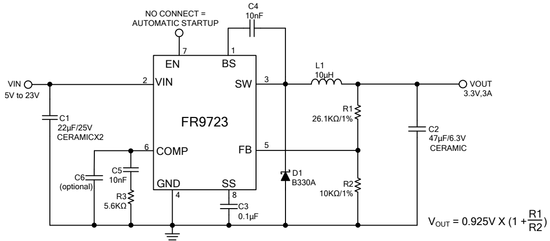
Figure 2. Output 3.3V Application Circuit
