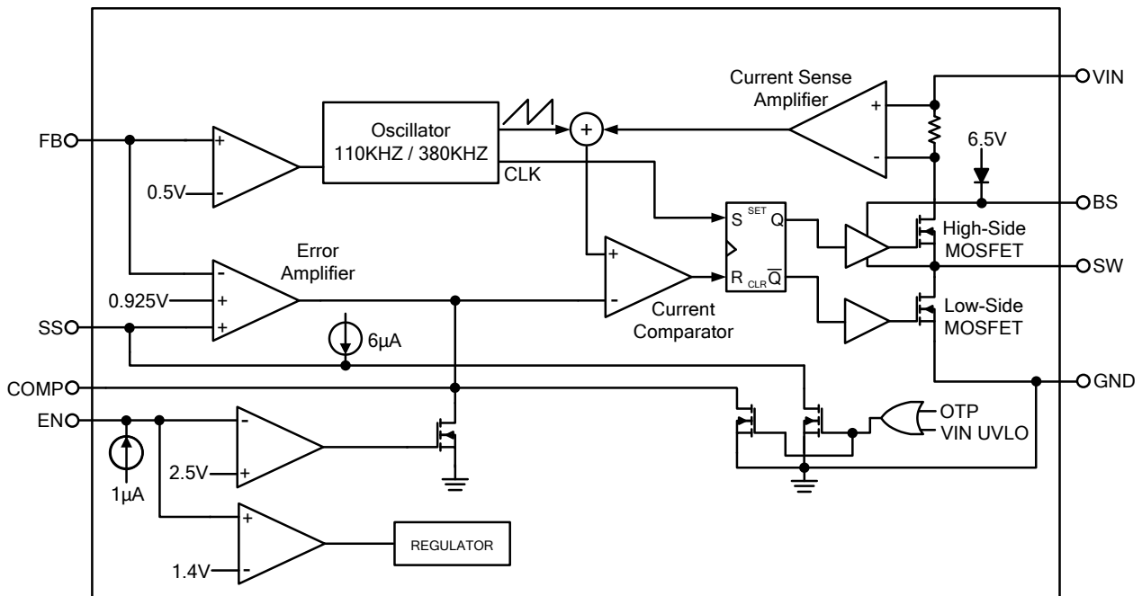
Figure 4. Block Diagram of FR9723
