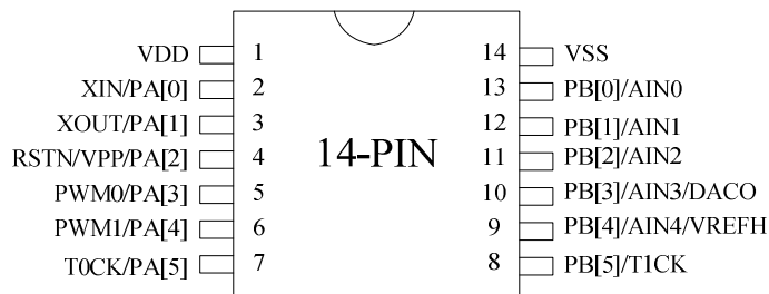
FM8PC71HM-A PDIP/SOP
