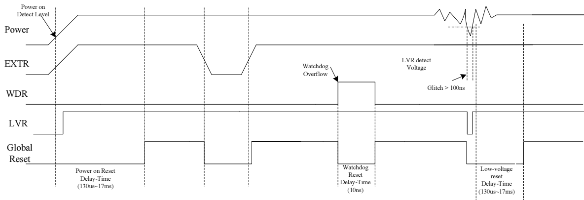
Figure 3.0-2 Global Timing
