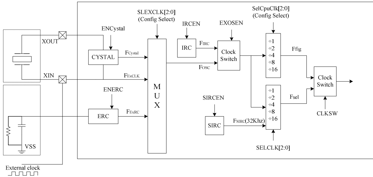
Figure 4.0-1 Clock Switch Block diagram
