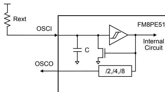
FIGURE 2.20: ERIC Oscillator Mode (External R, Internal C Oscillator)
