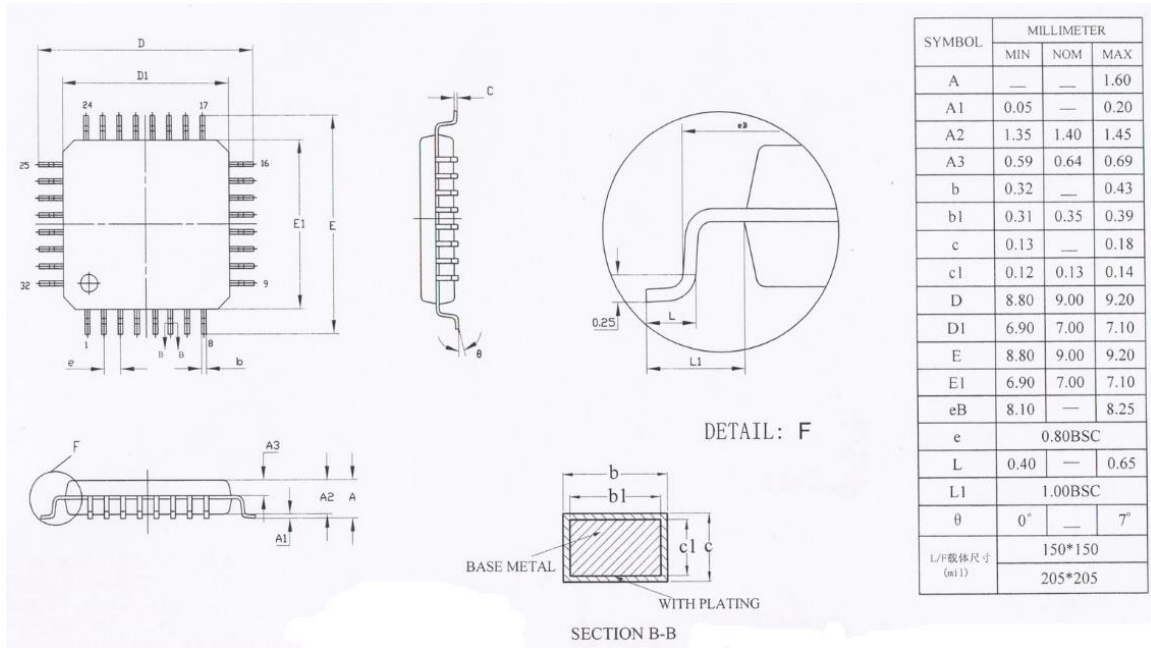
Figure 26-1 LQFP32 封装尺寸
